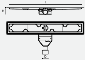
STL-DRAIN LOW H = 56 mm
