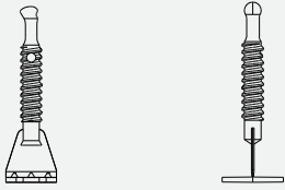
LEV/10 1 mm
