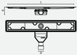
STL-DRAIN STANDARD H = 73 mm
