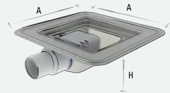
Removable siphon Stainless Steel Outlet of 40 mm diameter
