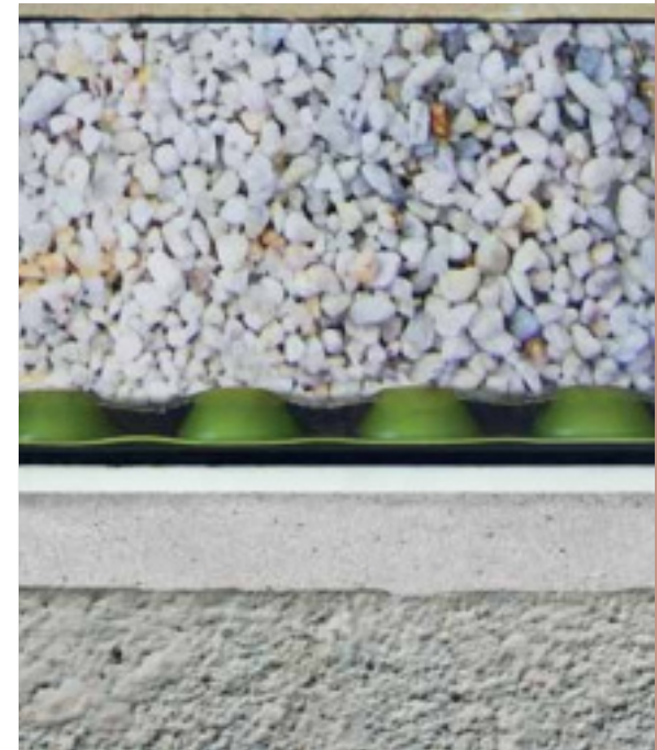
drain+tec 8s
